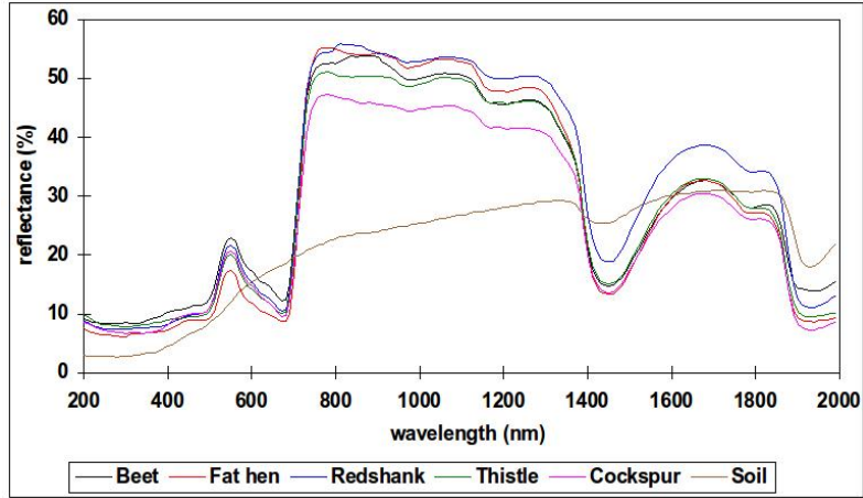
Figure 3: Spectral sensitivity of different plants and ground-types
