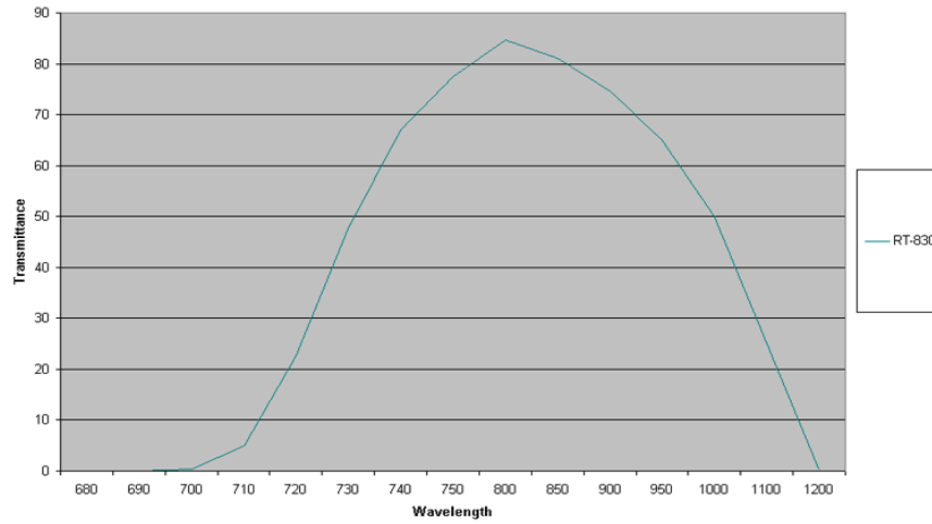
Figure 4: Spectral Diagram of the Hoya RT-830 filter
