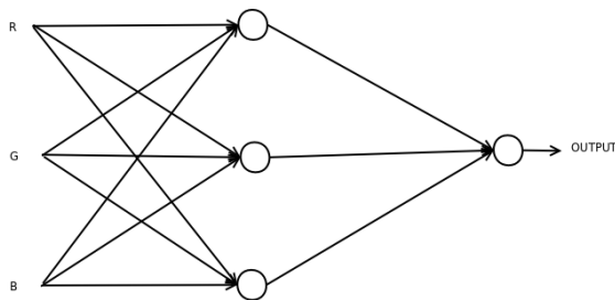
Figure 1: The neural network used in our experiment
