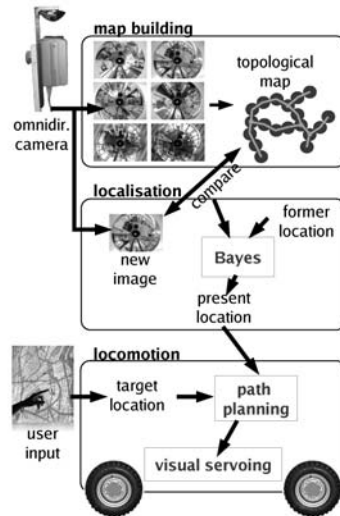
Figure 2: Overview of the navigation method
